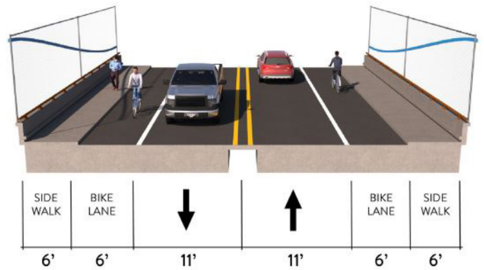
Preliminary rendering of Capitola Avenue Overcrossing
